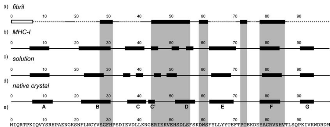
Figure 5. (a) Predicted \beta -strand regions (filled rectangles) in the fibrils, (b) \beta -strands in \beta_2m bound to the heavy chain in the MHC-I complex, 55 (c) \beta -strands in native \beta_2m as determined by solution NMR, 54 (d) \beta -strands in native monomeric \beta_2m as determined by X-ray crystallography, 56,57 and (e) the sequence of \beta_2m with all assigned residues in the fibril form underlined. The unfilled rectangle in (a) represents the dynamic N-terminus. The designation of each native strand is shown in (d).
