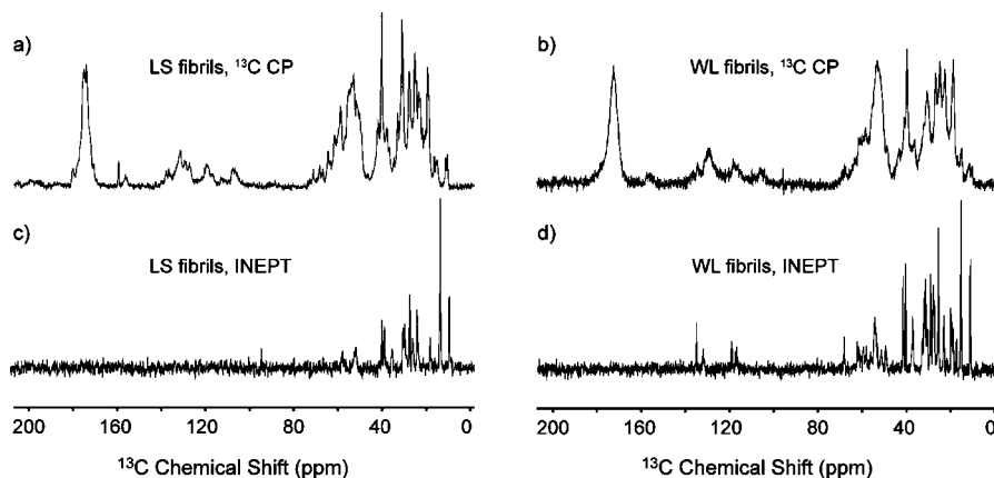
Figure 6. Comparison of CP (a and b) and INEPT (c and d) spectra of the LS U- \beta_2 m fibrils (a and c) and WL U- \beta_2 m fibrils (b and d). All spectra were obtained at 750 MHz in a 2.5 mm rotor (~5 mg of sample). The spectra in (a), (b), and (d) were recorded with \omega_r/2\pi = 12.5 kHz and 128 scans, while (c) was recorded with \omega_r/2\pi = 16.7 kHz with 32 scans.
