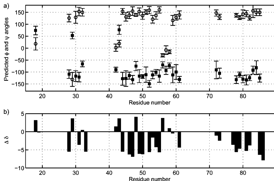
Figure 4. Chemical shift analysis of the LS fibril assignments based on (a) torsion angle analysis with TALOS and (b) the chemical shift index (CSI). The “○” symbols in (a) correspond to the predicted \Psi angles, while the “■” symbols correspond to the predicted \phi angles.
