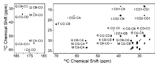
Figure 3. ^{13}\text{C} – ^{13}\text{C} INEPT-TOBSY spectrum obtained at 750 MHz and \omega_r/2\pi = 16.7 kHz with a \text{U-}\beta_2\text{m} LS fibril sample ( \tau_{\text{mix}} = 5.77 ms).
