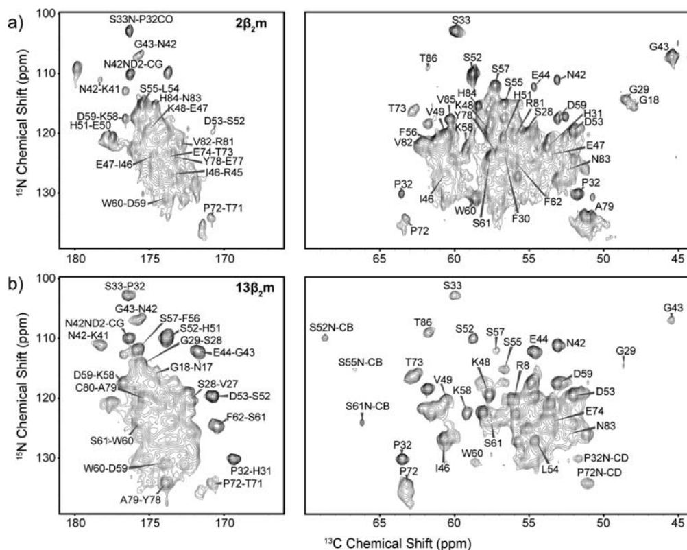
Figure 2. ^{15}\text{N} – ^{13}\text{C} correlation spectra of (a) 2\text{-}\beta_2\text{m} LS fibrils, obtained at 700 MHz, \omega_r/2\pi = 10.0 kHz, and (b) 1,3\text{-}\beta_2\text{m} LS fibrils, obtained at 750 MHz, \omega_r/2\pi = 12.5 kHz. Dipolar recoupling was achieved with ZF-TEDOR and \tau_{\text{mix}} = 1.6 ms. Unless otherwise noted, the labels refer to \text{N}_i\text{-CO}_{i-1} correlations (left panels) and \text{N}_i\text{-CA}_i correlations (right panels).
